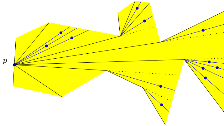
Figure 4: Computing a tree that contains a geodesic from p through every point of B' .
