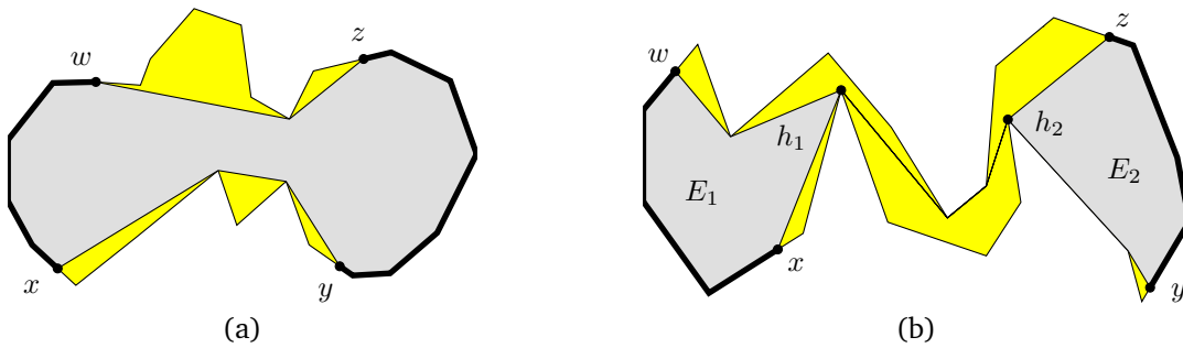
Figure 5: Two funnels: (a) a fat funnel and (b) a skinny funnel.
