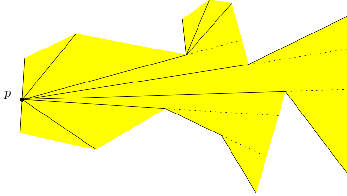
Figure 3: The augmented shortest path tree rooted at p . Edges added during the augmenting step are dotted.
