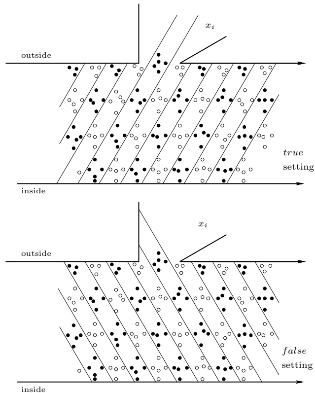
Figure 7: True and false settings of a variable.
