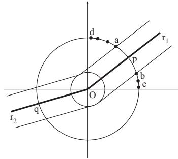
Figure 14: Lower bound for the widest anchored siphon.
