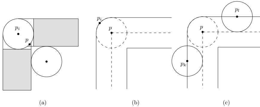
Figure 5: (a) The point p is a common vertex of two arcs of p_i in V(P, w) and H(P, w) . Notice that S_V(p_i) and S_H(p_i) (shaded rectangles) do not intersect. (b) and (c) two cases of an orthogonal siphon.
