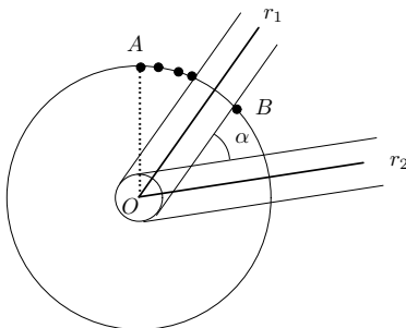
Figure 15: Lower bound for the widest anchored \alpha -siphon.
