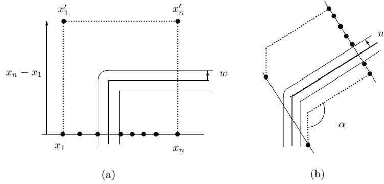
Figure 8: Lower bound for the oriented \alpha -siphon problem.
