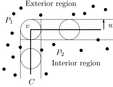
Figure 3: A S-E orthogonal siphon of width w .
