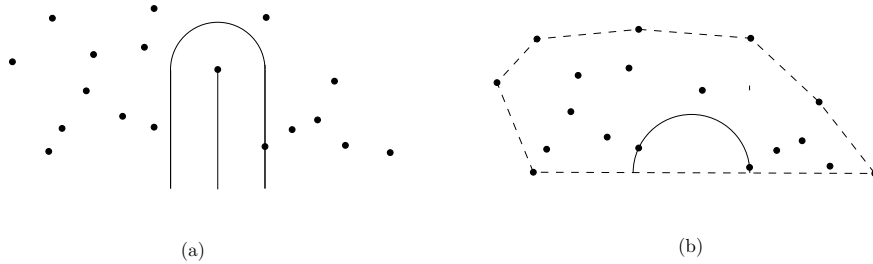
Figure 7: The oriented 0-siphon problem.
