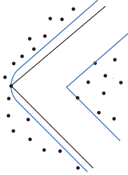
Figure 2: The width of the widest \alpha -siphon is larger than the width of the widest L-corridor.
