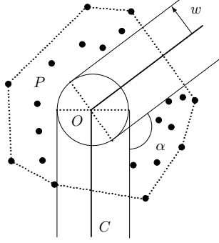
Figure 12: Anchored and arbitrarily-oriented \alpha -siphon.
