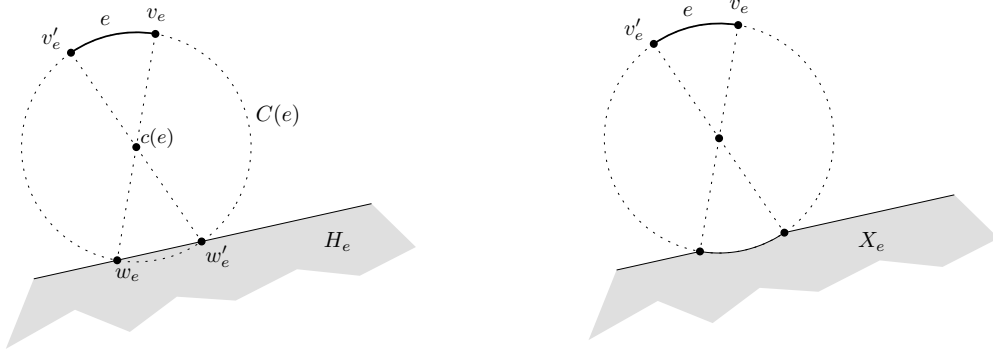
Figure 3: Left: notation concerning an edge e . Right: the region X_e .
