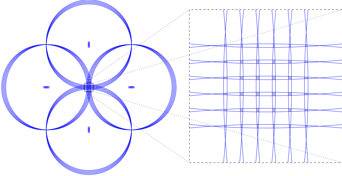
Figure 5: A collection of unit circles and a zoom to a part of the drawing. When the set of unit disks centered at points of B looks like in the figure, placing the center of the blue unit coin C_B in the grey faces of the arrangement would cover most points. A similar scenario but with red circles that is far enough gives rise to \Theta(n^4) optimal solutions to the Two-Coin Problem.
