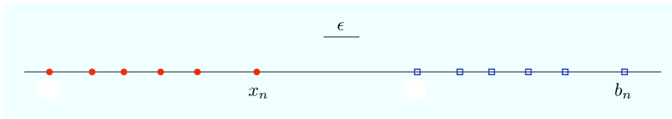
Figure 8: Red and blue points in the reduction for Theorem 6.
