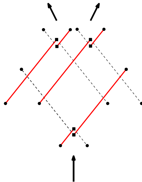
Figure 4: Splitter gadget.
