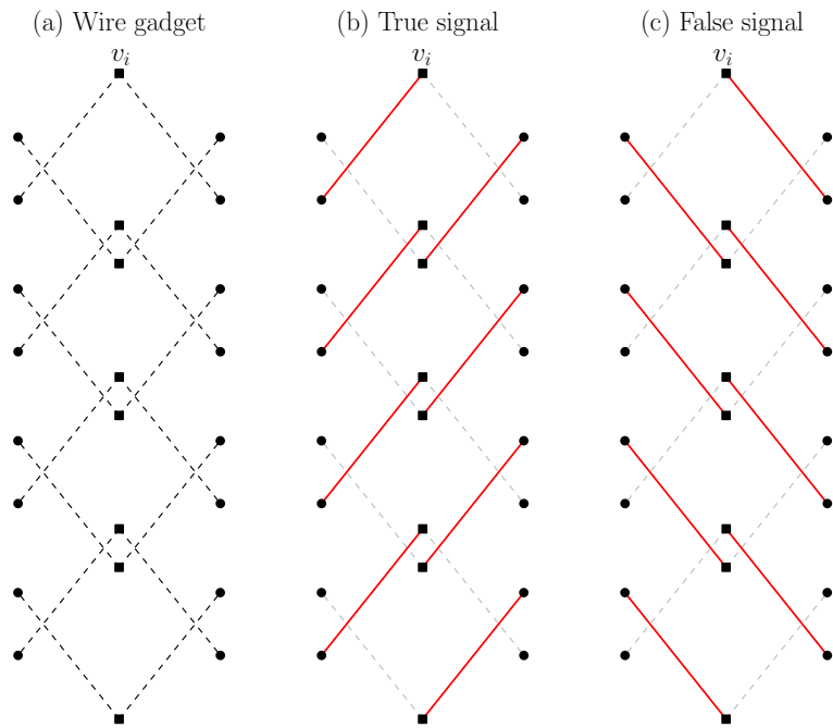
Figure 3: Wire gadget.
