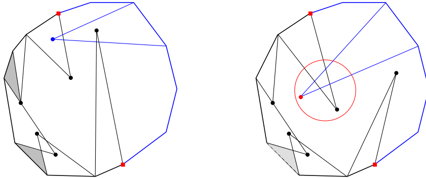
Figure 12: Merging two solved sub-problems. In the left diagram, the grey regions in the left (black) sub-problem cannot contain points from the right (blue) sub-problem if there is a valid solution. In the right diagram, we see the type of event that we must check for after some initial reductions.
